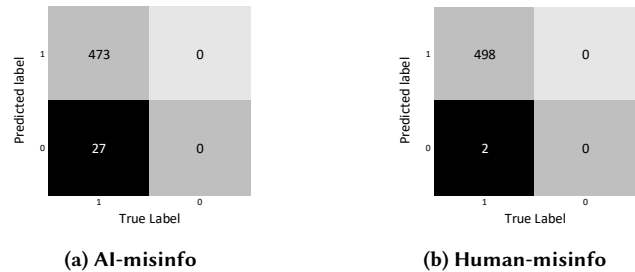
Figure 5: Confusion matrix for AI-misinfo and Human-misinfo datasets.
